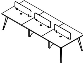
N20WSLS3S900120-2700 X 1200 X 1050 N20WSLS3S105120-3150 X 1200 X 1050 N20WSLS3S120120-3600 X 1200 X 1050
