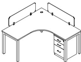
N550WSLS1S900120-900 X 1200 X 1050 N550WSLS1S105120-1050 X 1200 X 1050 N550WSLS1S120120-1200 X 1200 X 1050
